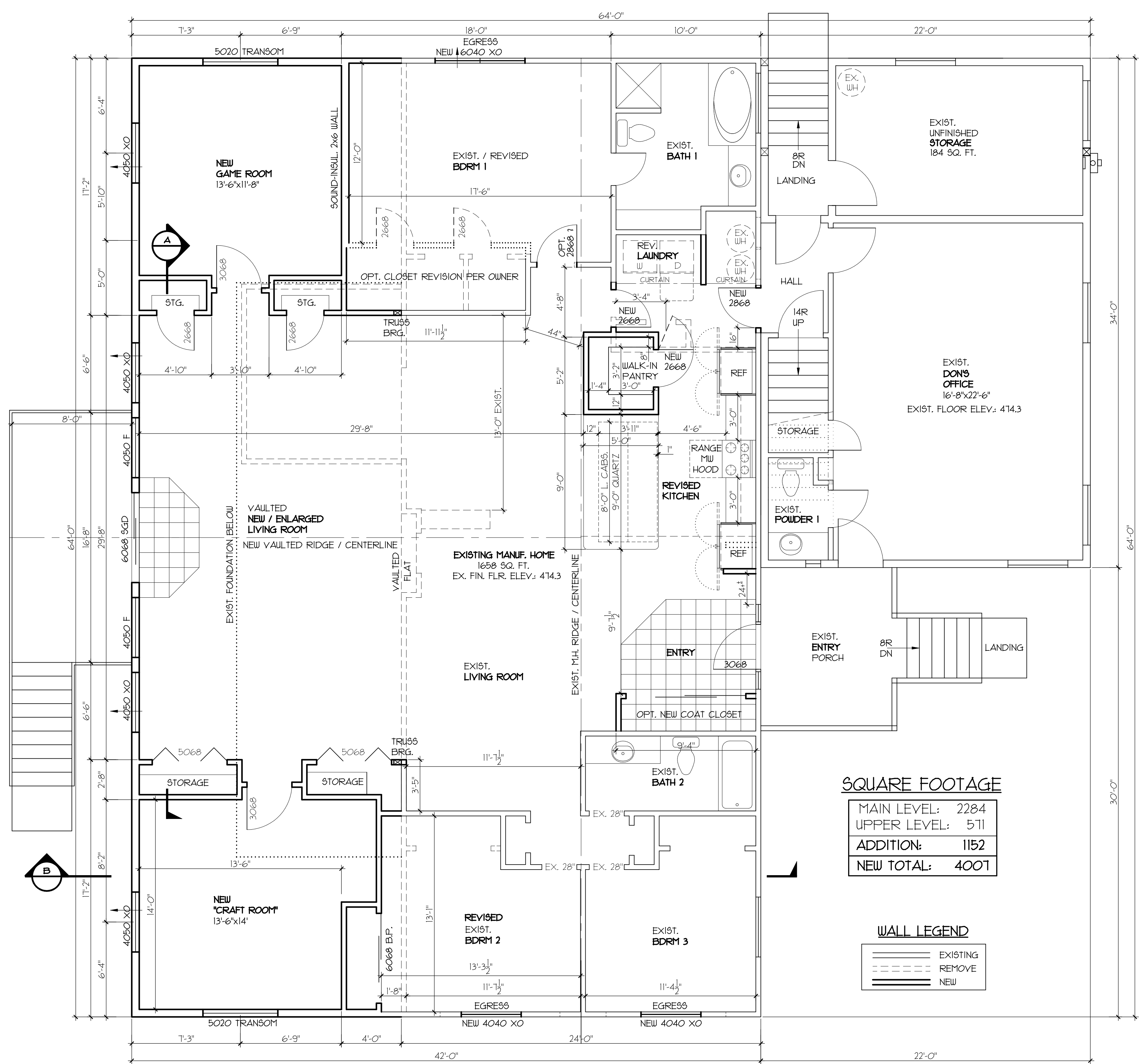
REVISED MAIN LEVEL FLOOR PLAN 1/4" = 1'-0"
