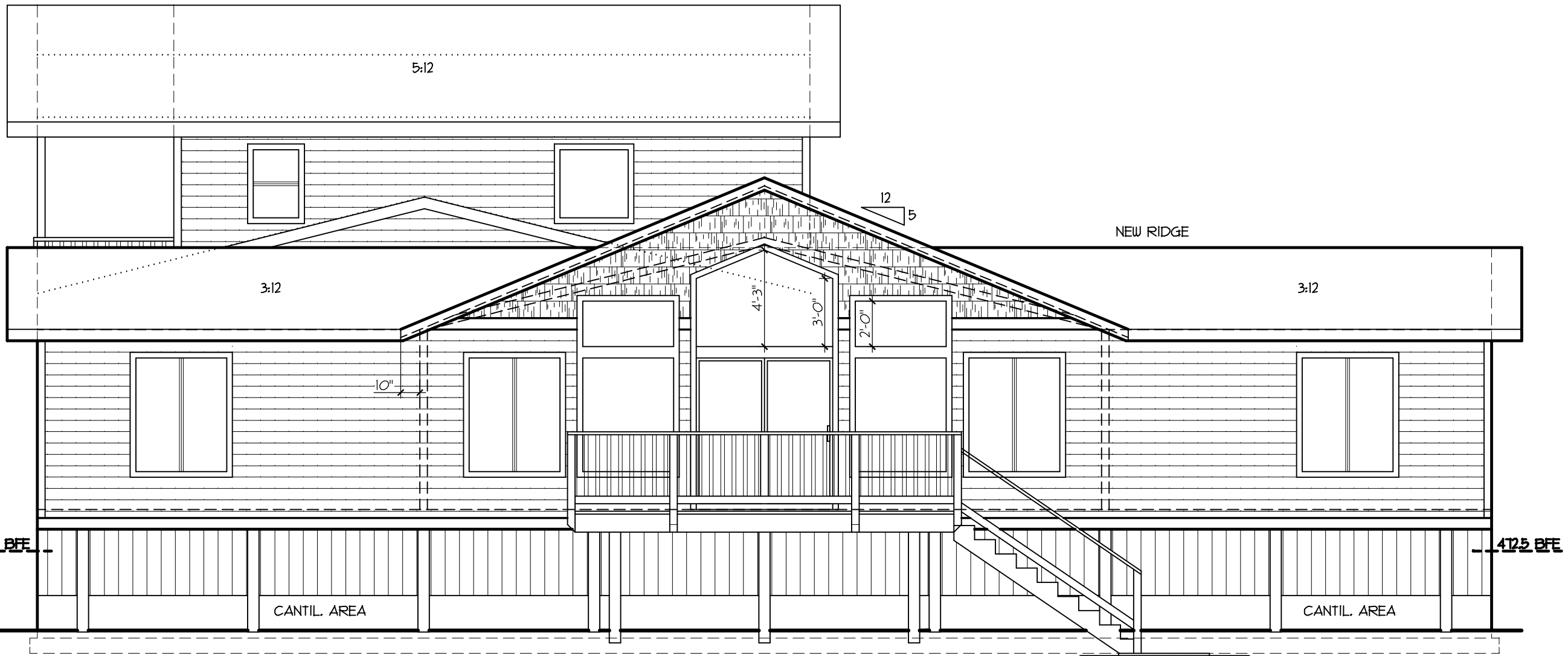
SOUTH LEFT ELEVATION 1/4" = 1'-0"
