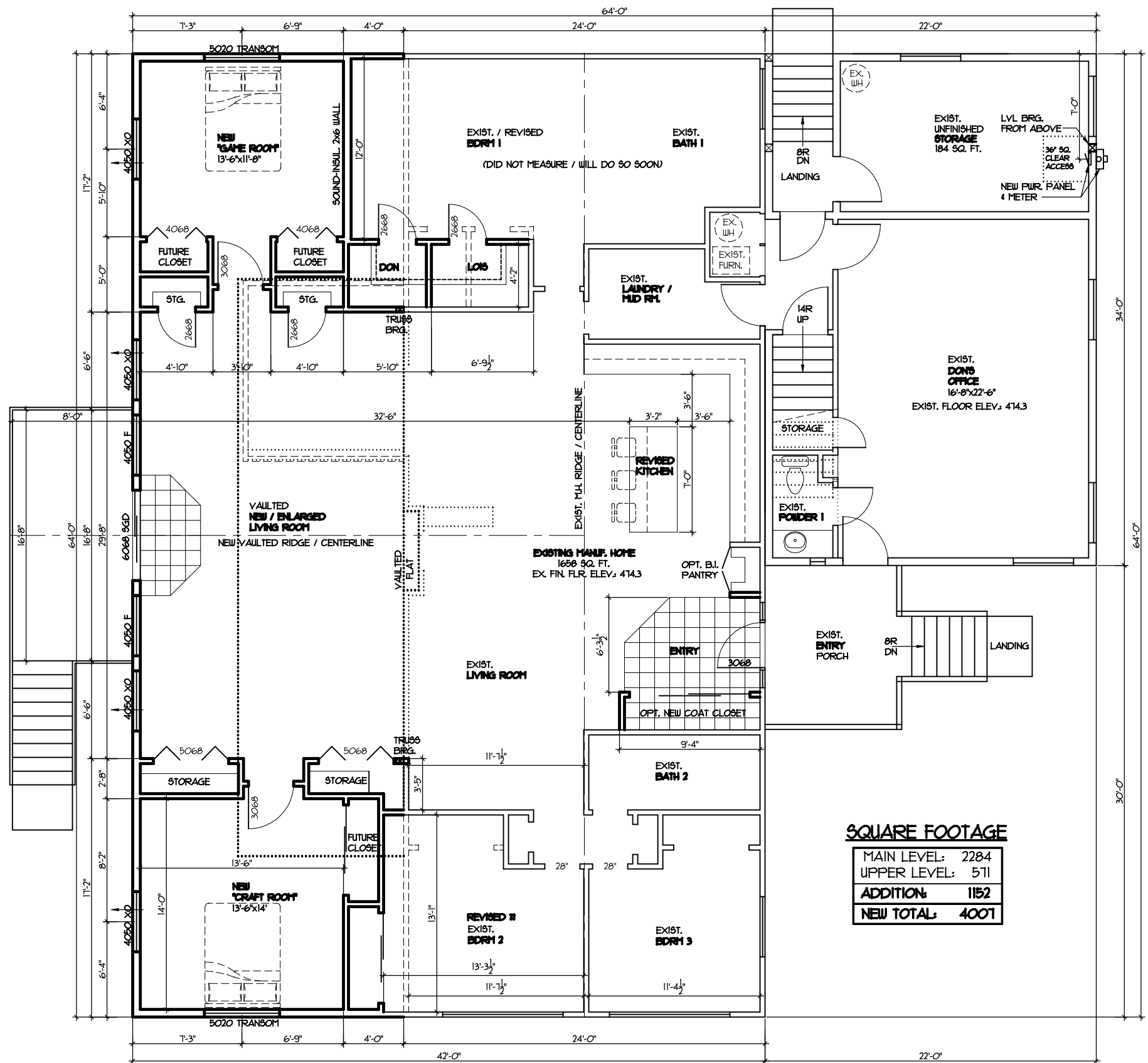
REVISED MAIN LEVEL FLOOR PLAN
