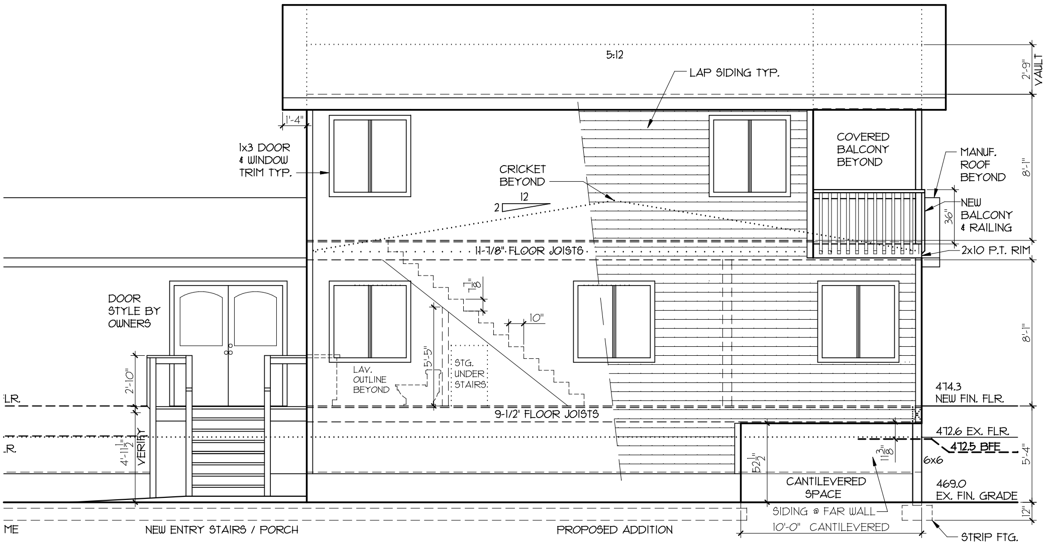
NORTH RIGHT ELEVATION 1/4" = 1'-0"
