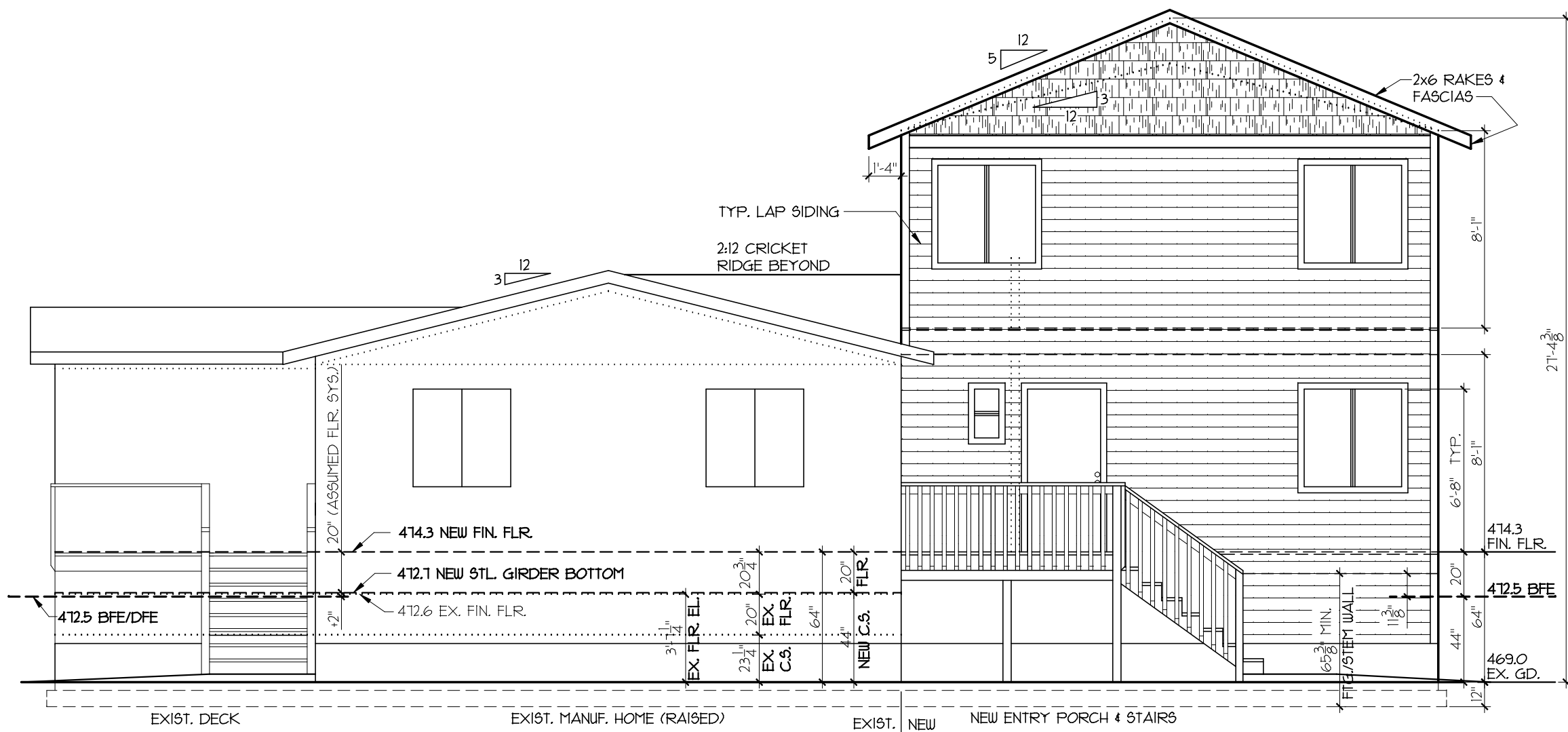
EAST (STREET VIEW) FRONT ELEVATION N.T.S.
