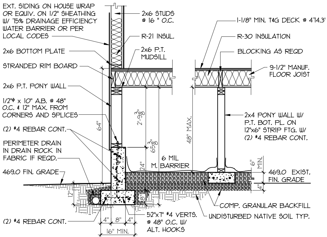
1 TYP. PERIMETER FOOTING DETAIL 1/2" = 1'-0"
