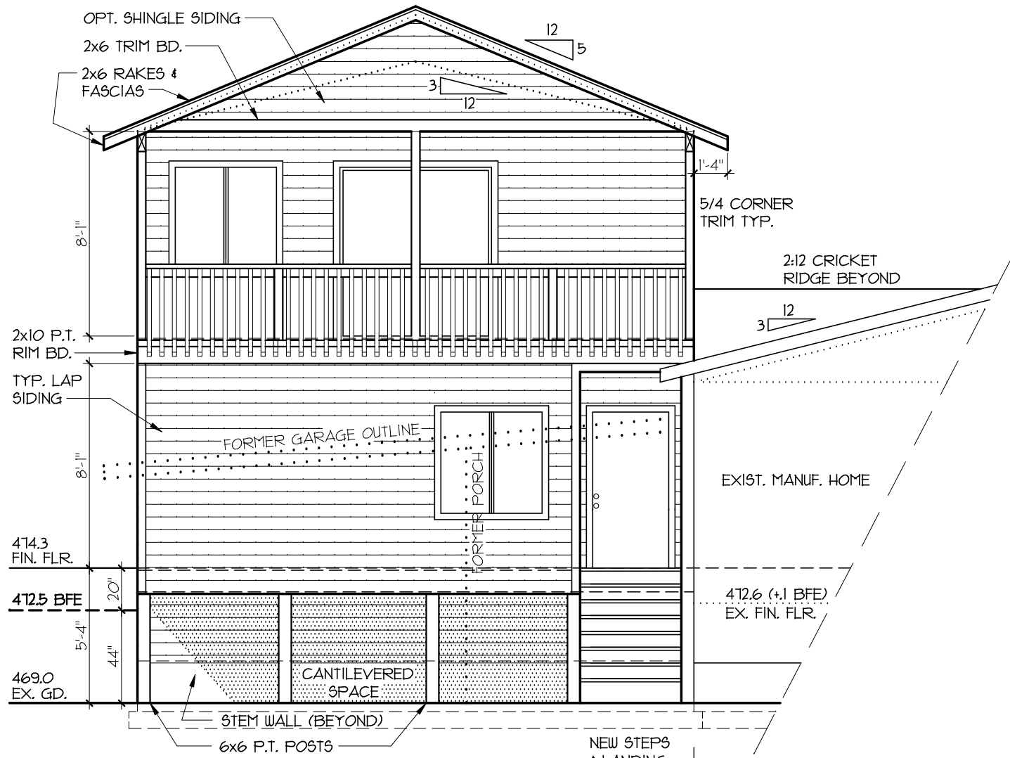
WEST REAR ELEVATION 1/4" = 1'-0" 8-5-13
