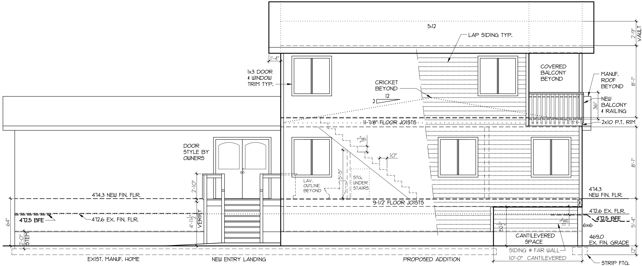
NORTH RIGHT ELEVATION 1/4" = 1'-0" 8-5-13
