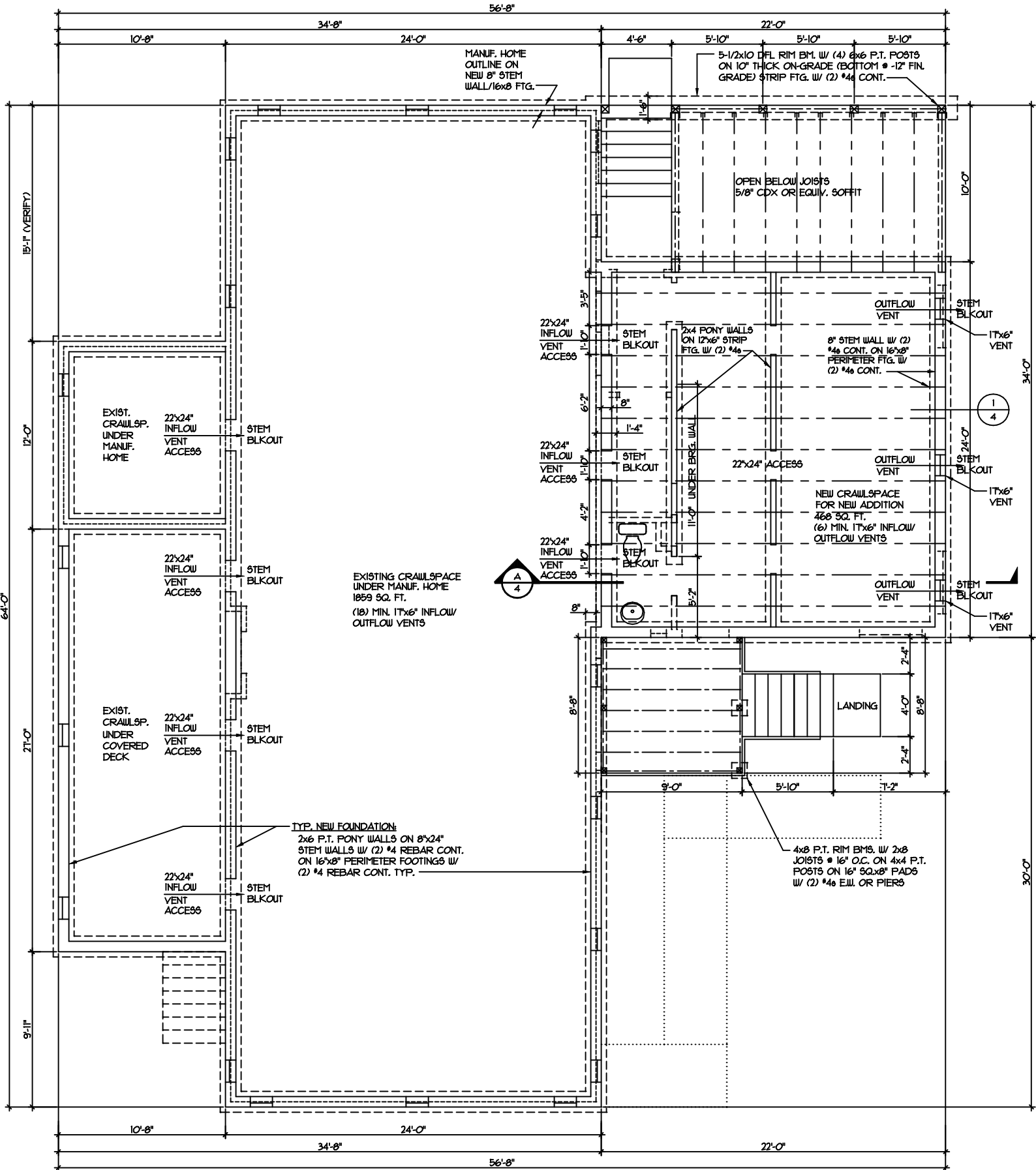
FOUNDATION PLAN 1/4" = 1'-0"
