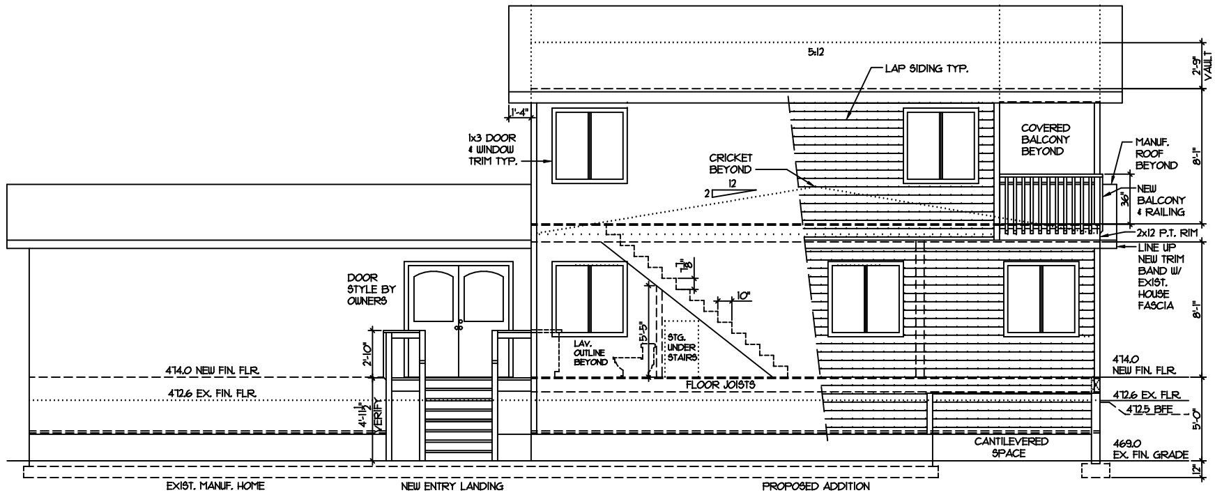
NORTH RIGHT ELEVATION 1/4" = 1'-0"
