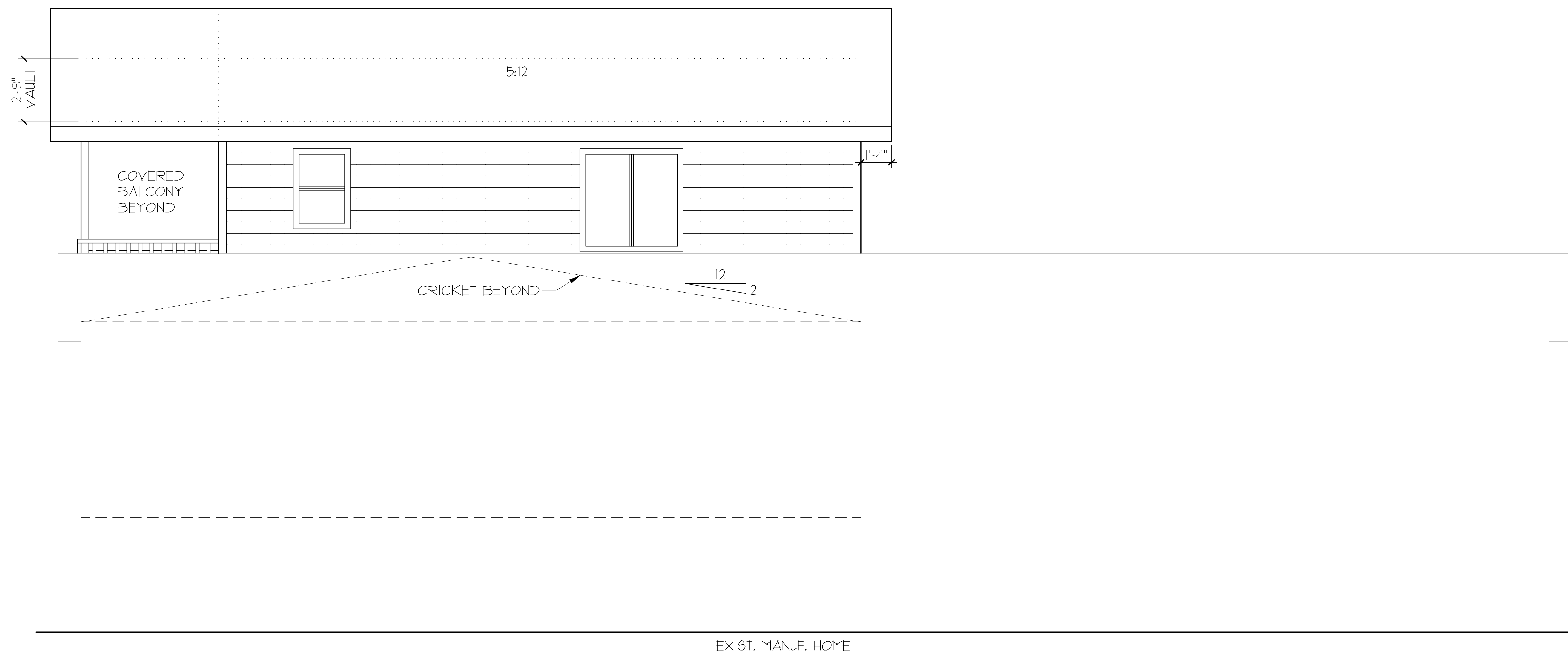
LEFT ELEVATION 1/4" = 1'-0"
