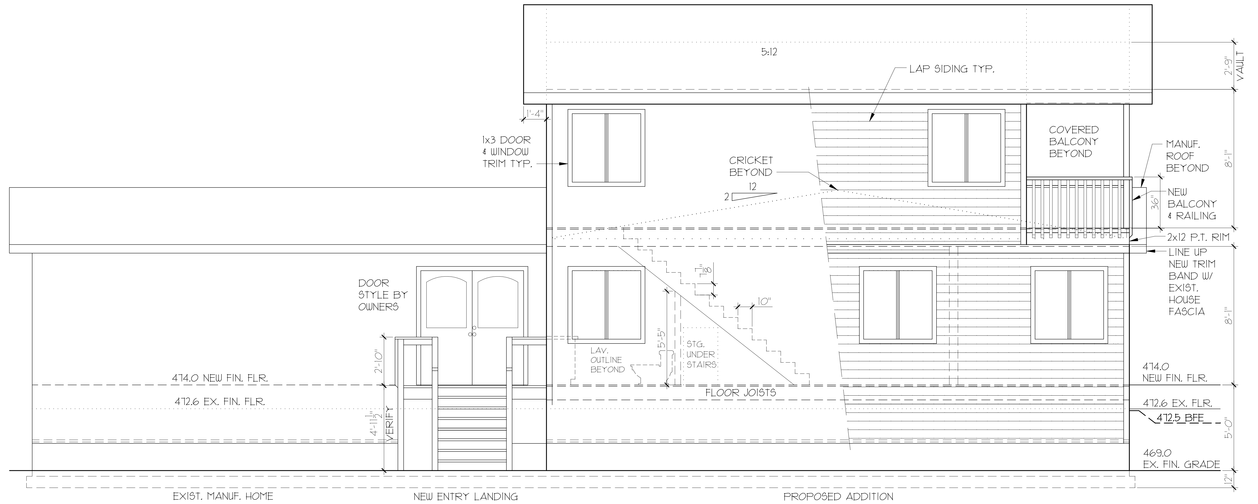
NORTH RIGHT ELEVATION 1/4" = 1'-0"
