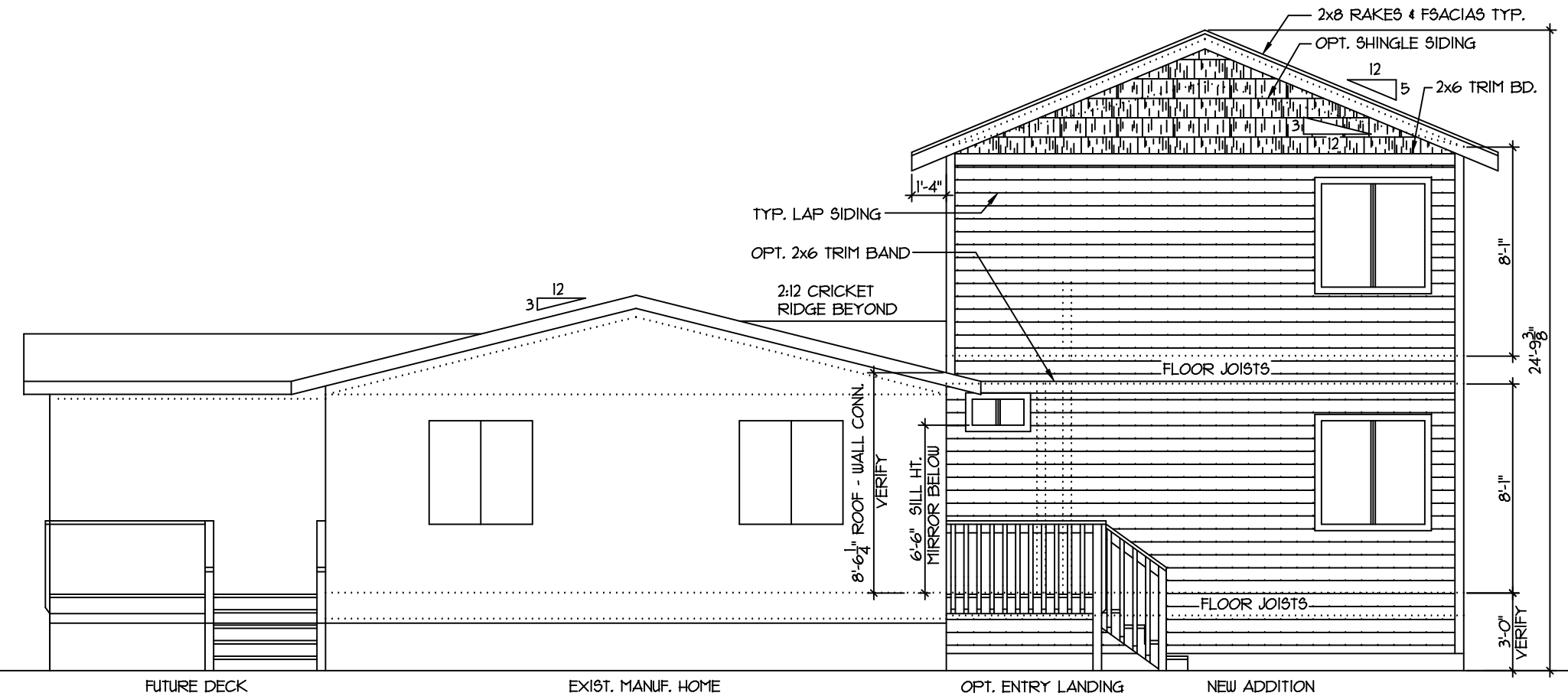
STREET VIEW FRONT ELEVATION 1/4" = 1'-0"
